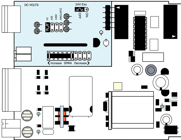
Main PCB*
