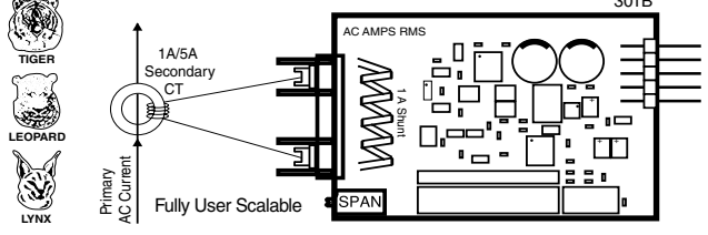
IA10: AC Millivolts, Scaled RMS, 100mV AC
