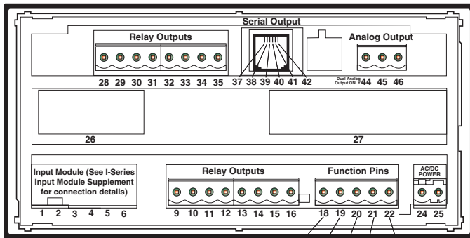
Rear Panel
