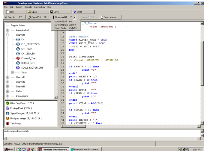
Tiger Development System screen showing the compiled Macro being downloaded into a Tiger 320 Series PMC.
