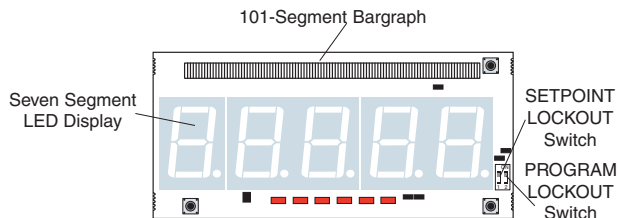
Display PCB without Faceplate and Bezel
