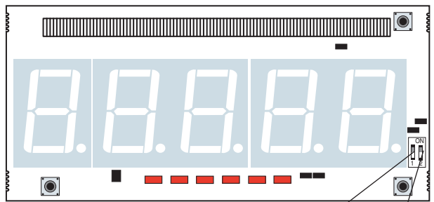
Display Board
