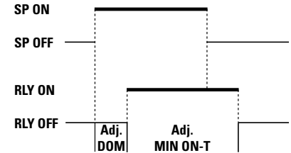
Figure 25 – 1-Shot ON Mode
