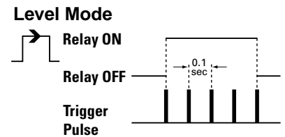
Figure 36 – Level Mode
