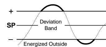
Figure 13 – Deviation Delay
