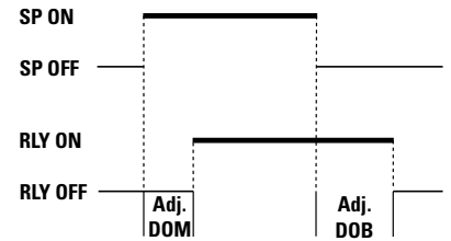
Figure 19 – Normal Mode
