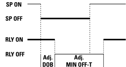
Figure 27 – 1-Shot OFF Mode
