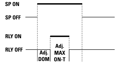
Figure 23 – Pulse ON Mode
