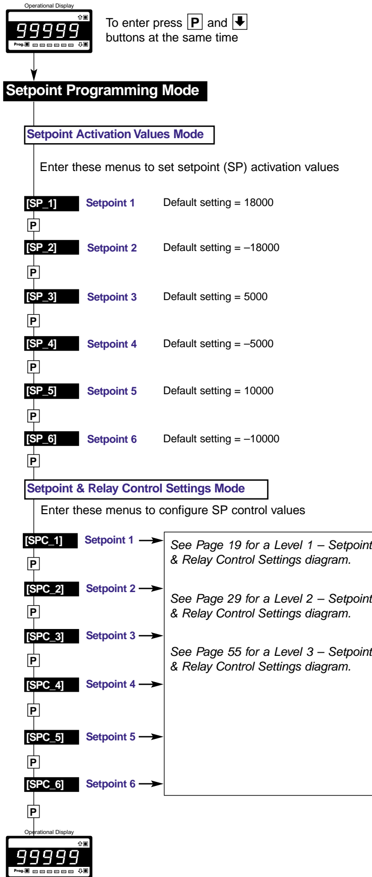
Figure 3 – Setpoint Programming Mode Logic Diagram
