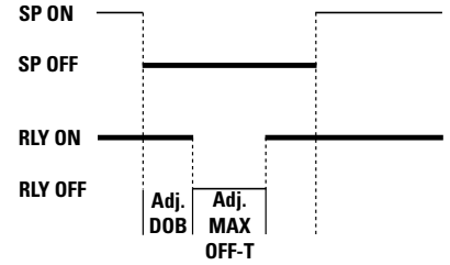
Figure 29 – Pulse OFF Mode
