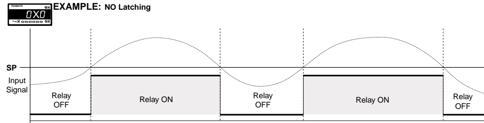
Figure 5 – NO Latching
