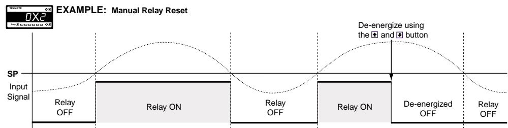
Figure 7 – Manual Relay Reset
