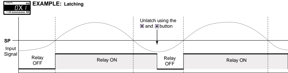
Figure 6 – Setpoint Latching
