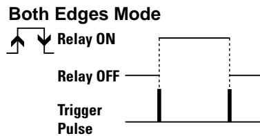
Figure 35 – Both Edges Mode
