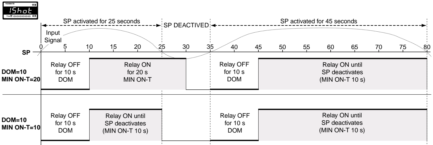
Figure 26 – 1-SHOT ON Mode Time Control
