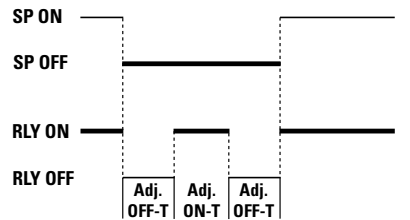
Figure 31 – Repeat OFF Mode
