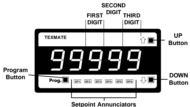
Figure 2 – Meter Programming Digits for Setpoint and Relay Control Functions
