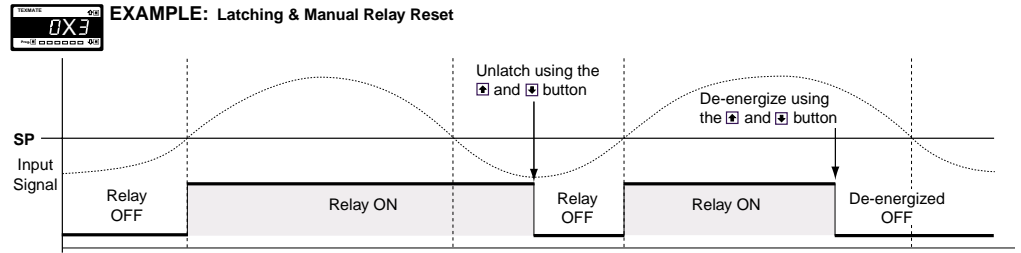
Figure 8 – Latching & Manual Relay Reset
