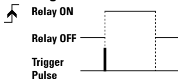
Figure 33 – Make Edge Mode
