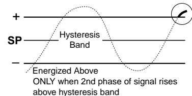
Figure 11 – Hysteresis Delay
