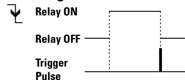
Figure 34 – Break Edge Mode
