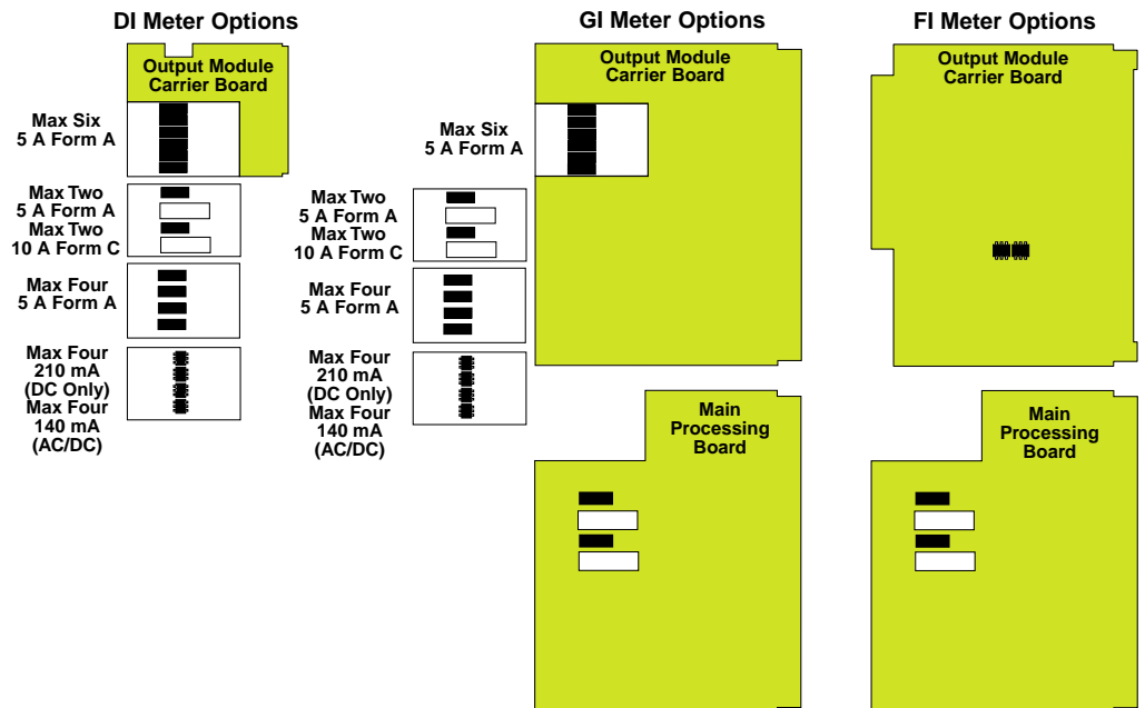
Figure 4 – Tiger 320 Series Relay Options
