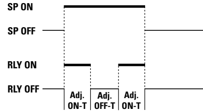
Figure 21 – Repeat ON Mode
