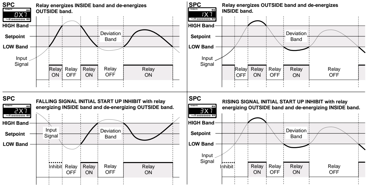
Figure 14 – Example 2: Relay energize functions with deviation
