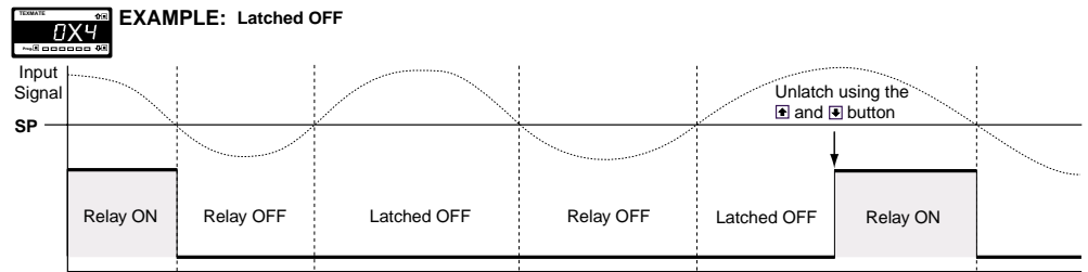
Figure 9 – Latched OFF
