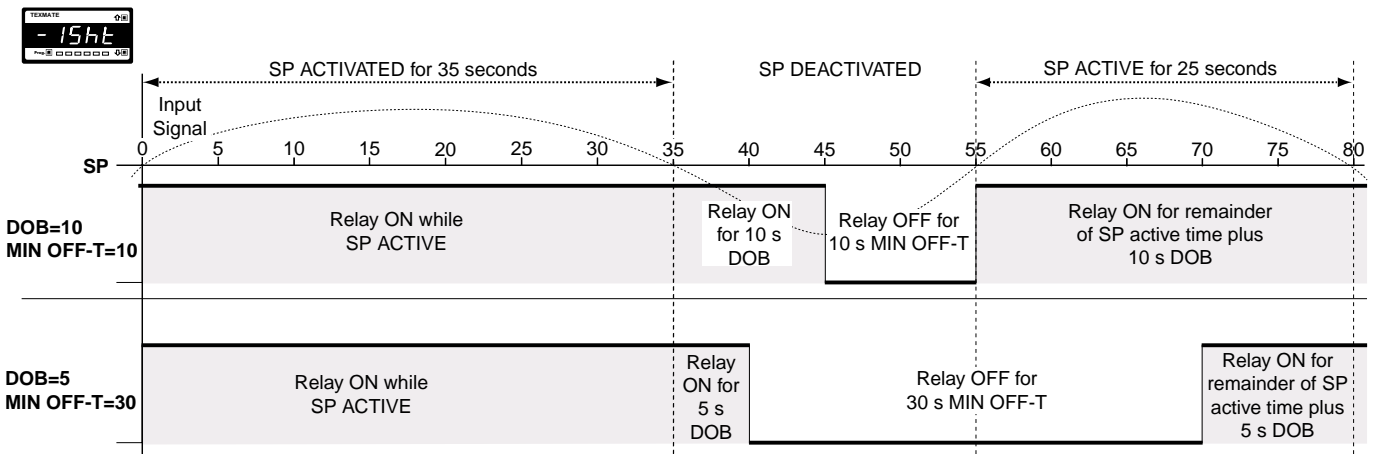
Figure 28 – 1-Shot OFF Mode Time Control
