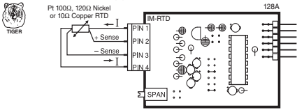
IT03: RTD, 100Ω Pt. 2/3/4-wire (-200 to 800°C) IT04: RTD, 100Ω Pt. 2/3/4-wire (-200 to 1470°F) IT05: RTD, 100Ω Pt. 2/3/4-wire (-199.9 to 199.9°F) IT14: RTD, 100Ω Pt. 2/3/4-wire (-199.9 to 199.9°C)
