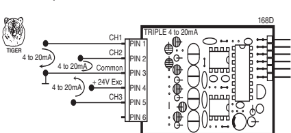
ITP1: Triple 4 to 20mA
