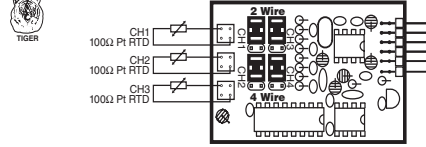
ITT2: Triple RTD Platinum 100Ω RTD 2 Wire Connection
