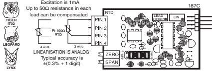
IT03: RTD, 100Ω Pt. 2/3/4-wire (-200 to 800°C) IT04: RTD, 100Ω Pt. 2/3/4-wire (-200 to 1470°F) IT05: RTD, 100Ω Pt. 2/3/4-wire (-199.9 to 199.9°F) IT14: RTD, 100Ω Pt. 2/3/4-wire (-199.9 to 199.9°C)
