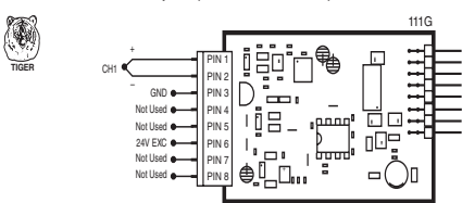
IT02: RTD, 100Ω Pt. 2/3/4-wire IT12: RTD, 120Ω Nickel 2/3/4-wire IT13: RTD, 10Ω Copper 2/3/4-wire
