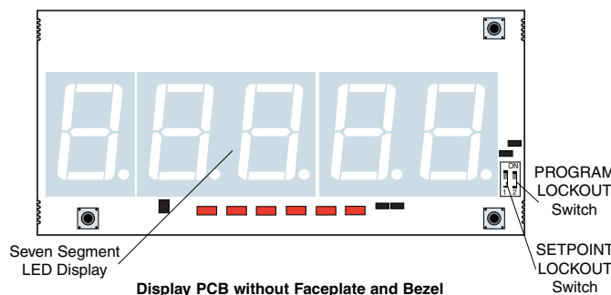
Display PCB without Faceplate and Bezel
