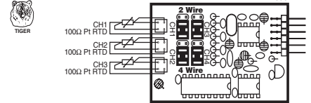
ITTC: Triple RTD Platinum 100Ω RTD 4 Wire Connection
