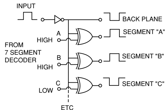
FIGURE 4. Exclusive-Or Drive Circuit
