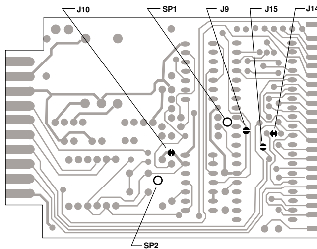
SOLDER SIDE
