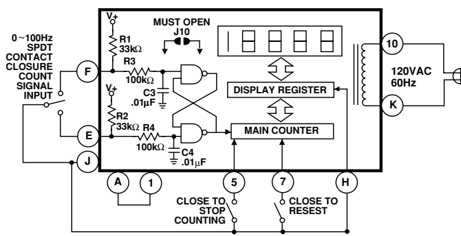
DOUBLE CONTACT CLOSURE COUNT INPUT
