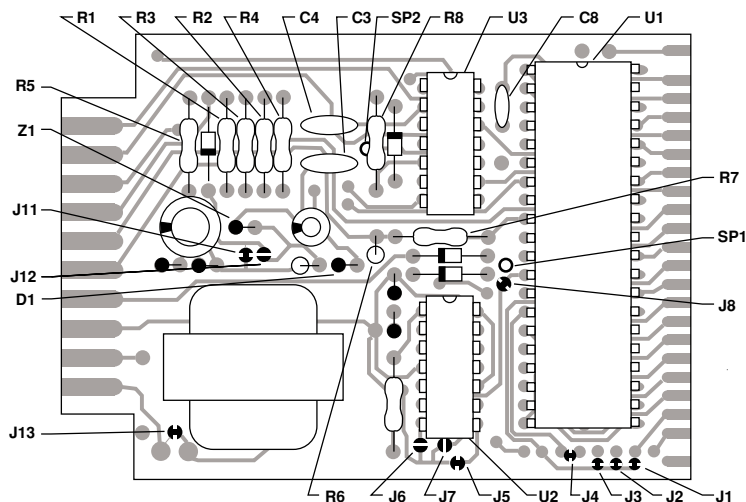
COMPONENT SIDE
