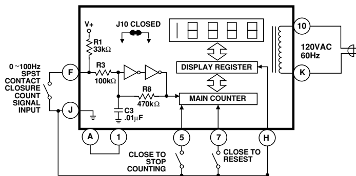
COUNT INPUT WITH SINGLE CONTACT SWITCH CLOSURE
