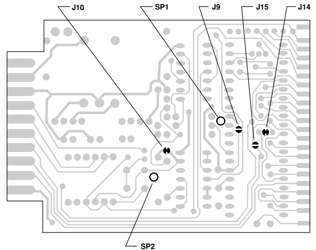
SOLDER SIDE
