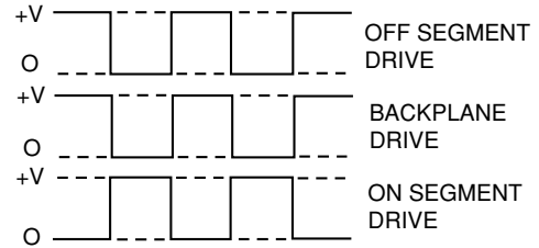
FIGURE 3. Typical AC Drive Signals
