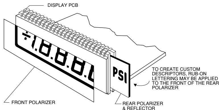
FIGURE 5. Replaceable Polarizers & Reflector Assembly
