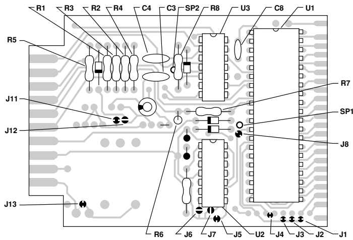
COMPONENT SIDE
