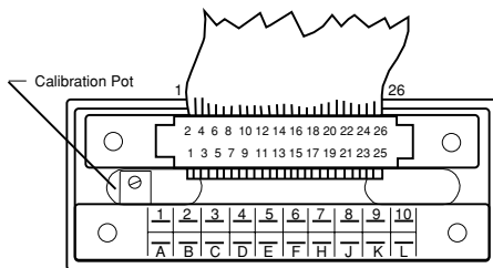
REAR VIEW OF METER CASE
