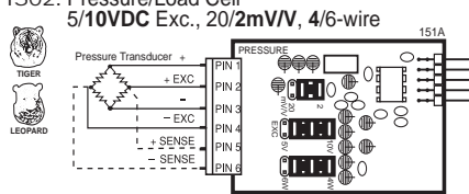
ISO2: Pressure/Load Cell 5/10VDC Exc., 20/2mV/V, 4/6-wire
