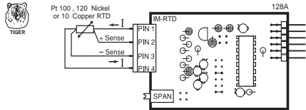
IT03: RTD, 100 Pt. 2/3-wire (-200 to 800°C) IT04: RTD, 100 Pt. 2/3-wire (-200 to 1470°F) IT05: RTD, 100Ω Pt. 2/3-wire (-199.9 to 199.9°F) IT14: RTD, 100Ω Pt. 2/3-wire (-199.9 to 199.9°C)
