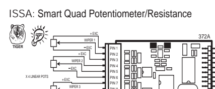
ISSA: Smart Quad Potentiometer/Resistance
