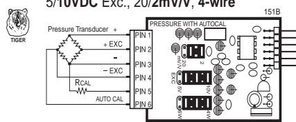
ISO3: Pressure/Load Cell with AutoCal 5/10VDC Exc., 20/2mV/V, 4-wire
