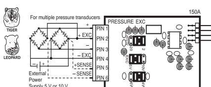
ISO4: Pressure/Load Cell Ext Exc., 20/2mV/V, 4/6-wire
