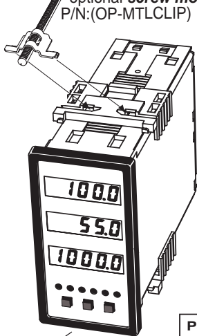
Metal Surround Case (P/N: OP-MTL96X48)
