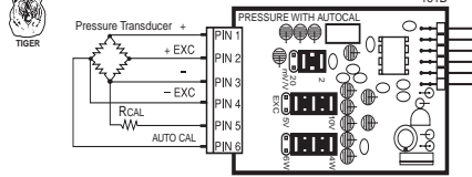
ISO4: Pressure/Load Cell Ext Exc., 20/2mV/V, 4/6-wire
