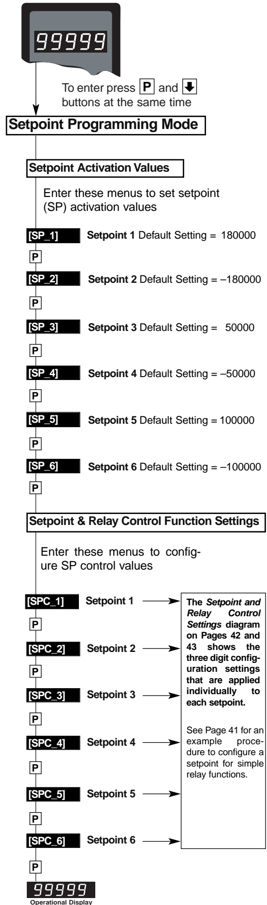
Setpoint Programming Mode Logic Diagram
