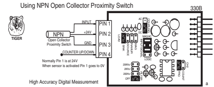
TTL Input Connected to IF10
