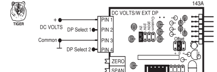
ID06: DC Volts 2/20/200/Custom V DC with External Decimal Select
