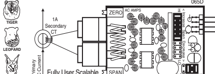
IA05: AC Amps Scaled RMS, 5 Amp AC
