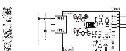
IA06: AC Volts True RMS, 300/600V AC
