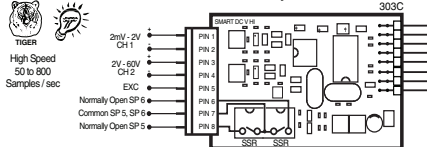
ISD1: Smart DC Volts. 16 bit. Optimized for 50 Hz rejection ISD2: Smart DC Volts. 16 bit. Optimized for 60 Hz rejection ISD3: Smart DC Volts. 16 bit. 50 Hz rejection w/dual SSRs. ISD4: Smart DC Volts. 16 bit. 60 Hz rejection w/dual SSRs.
