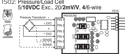
IS02: Pressure/Load Cell 5/10VDC Exc., 20/2mV/V, 4/6-wire
