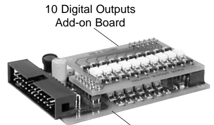
Standard 6 Digital Inputs/6 Digital Outputs
