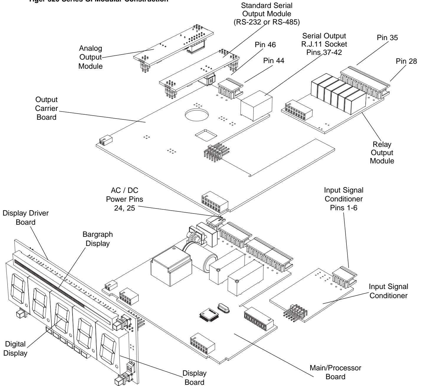
Exploded View of Meter Modular Boards
