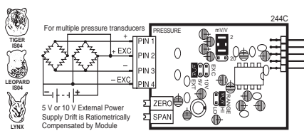
IS06: Pressure/Load Cell Ext Exc., 20/2mV/V, 4-wire
