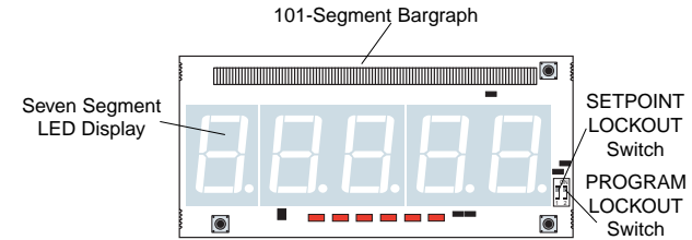
Display PCB without Faceplate and Bezel
