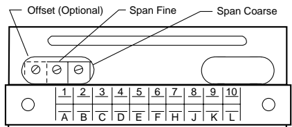
REAR OF METER WITH PCB EDGE CONNECTOR MOUNTED (For mounting of screw terminal blocks see below)
