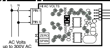
AC Voltage measurement in Single-phase Systems.
