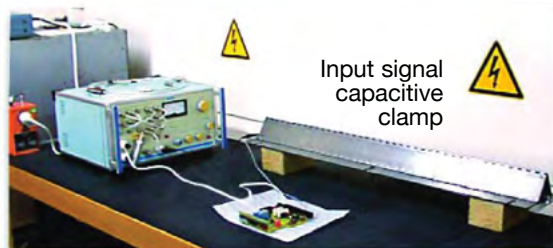
NOISEKEN Burst Testing, Direct and Coupled. Selectable pulse width from 50nS to 1.2μS at 0 to 100Hz with sub nano sec rise time.
