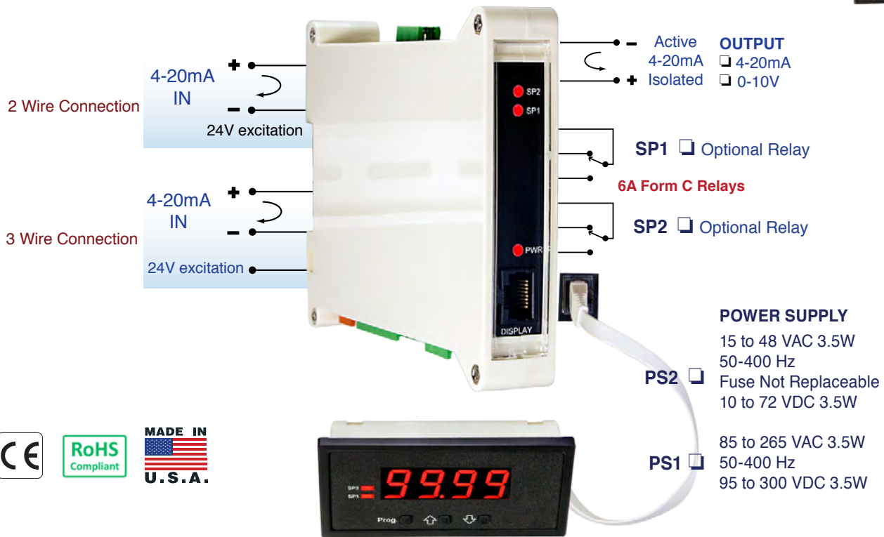
Optional Remote Display Programmer Needed for Programming Relays
