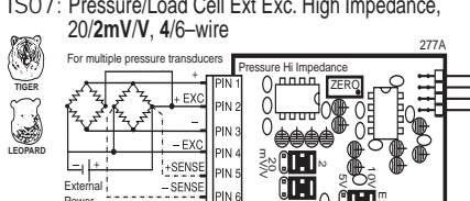
IS07: Pressure/Load Cell Ext Exc. High Impedance, 20/2mV/V, 4/6-wire
