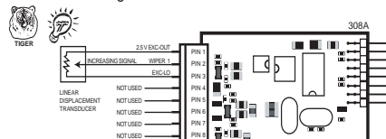
ISR3: Smart Dual 3-Wire Potentiometer. 16 bit. 50 Hz
