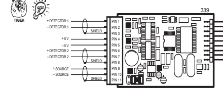
ISSE: Smart Dual Photo Diode Input
