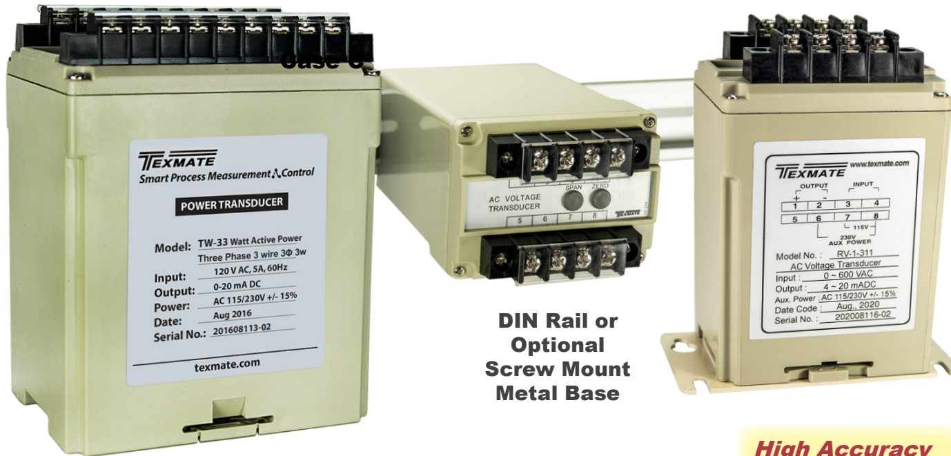
Fire-Retardant ABS DIN Rail Mount Case
